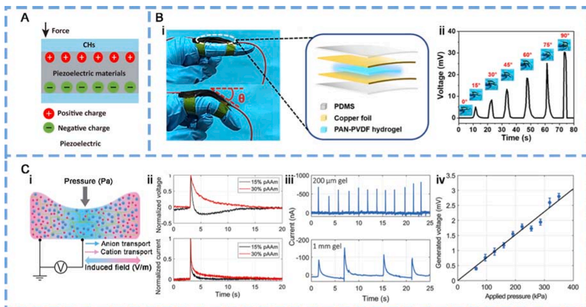
Fig. 12. CHs-based piezoelectric nanogenerators (PENGs). (A) Working mechanism of CHs-based PENGs. (B) Structure i) of CHs-based PENG for bioenergy harvesting and ii) its output. Reproduced from ref. [327] with permission from American Chemical Society, copyright 2019. (C) i) Schematic of a polymer gel under indentation, exhibiting differential ionic displacement and field. ii) Piezoionic transient response under a step compression for 15 and 30% pAAm swollen in 1.5 M NaCl. iii) Piezoionic transient response under repeated step compressions onto a 200-μm-thick (top) and a 1-mm-thick (bottom) pAAm gel swollen with 1.5 M NaCl, exhibiting decay times of ~ 50 ms and ~ 5 s, respectively. iv) Peak generated voltage as a function of applied pressure (data are mean ± SD, N = 3). Reproduced from ref. [328] with permission from American Association for the Advancement of Science, copyright 2022.
