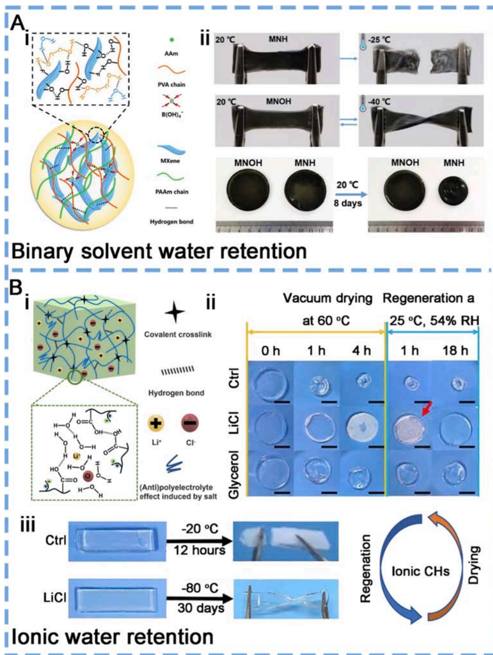
Fig. 4. Water retention ability. (A) Binary solvent anti-freezing CHs. i) Schematic illustration of the fabrication of a CH with good water retention ability. ii) Photographs of anti-freezing and long-lasting moisture retention performance. Reproduced from ref. [141] with permission from Springer Nature Limited, copyright 2021. (B) Ion dropping water retention CHs. i) Images of control, glycerol-based, LiCl-based hydrogels stored at 25 °C and 54% RH for 0 and 7 days. ii) Compressive modulus of original LiCl-based hydrogels and the ones stored at 25 °C and 54% RH for 7 days. iii) Twist of control or 30% LiCl-based hydrogels subjected to subzero temperature for a determined period. Reproduced from ref. [145] with permission from Elsevier, copyright 2021.
