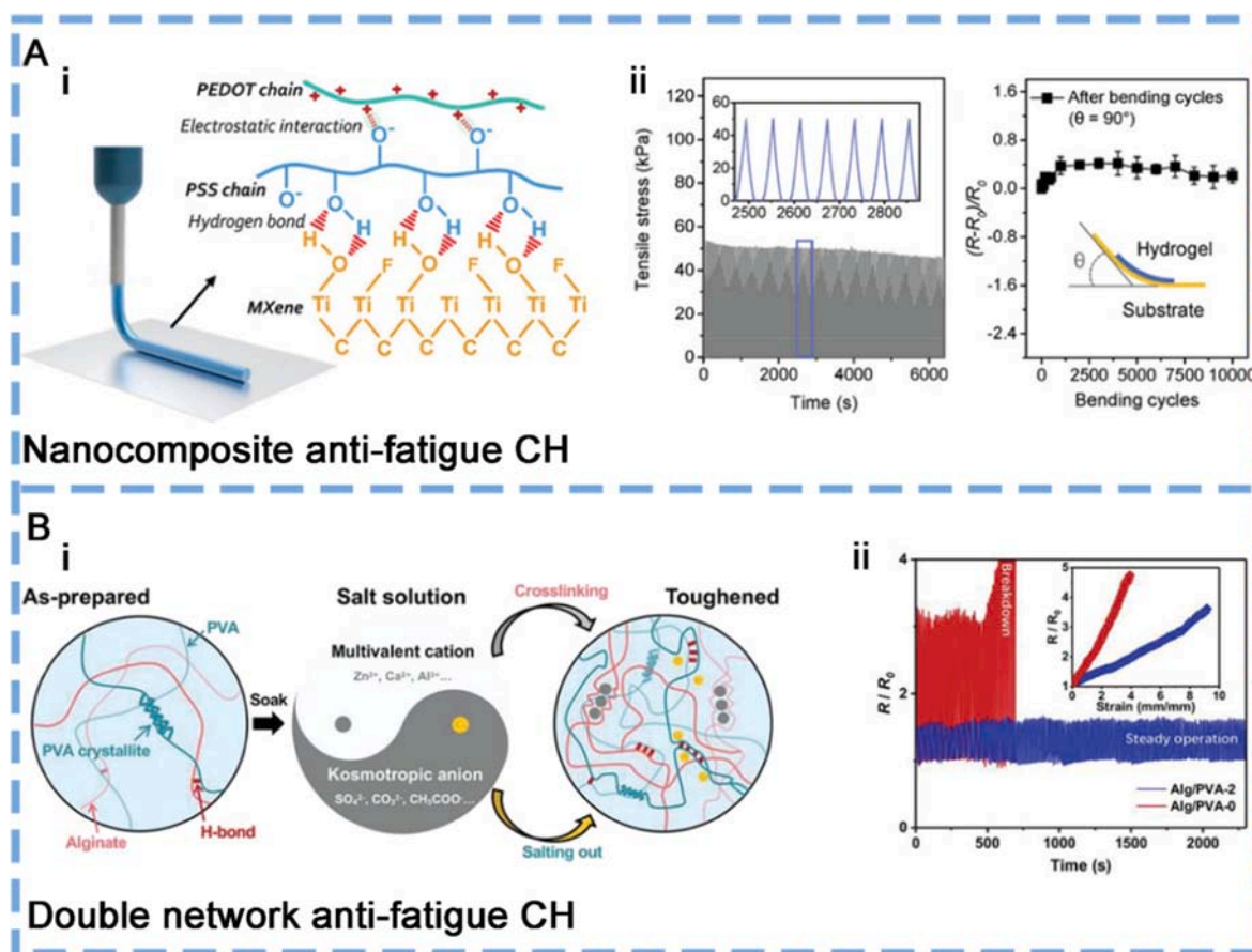
Fig. 10. Representative sample to composite CHs with good fatigue stability. (A) Nanocomposite anti-fatigue CH i) Scheme illustrating the preparation of MXene-functionalized PEDOT:PSS ink for extrusion printing. ii) The tensile stress–strain curves of the printed hydrogel at a strain of 5% for >100 cycles and electrical resistance variations as a function of bending cycles ( 90^\circ ). Reproduced from ref. [13] with permission from Wiley-VCH, copyright 2022. (B) Ionic reinforcement of anti-fatigue CH. i) Schematic diagram of the synthesis of PVA ion-reinforced CHs. ii) Cyclic performance of the notched sensor at a strain of 200%. Reproduced from ref. [270] with permission from Wiley-VCH, copyright 2022.
