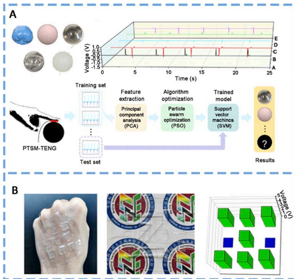
Fig. 18. (A) Glove-based human-computer interaction (HMI) system using ionic hydrogel-based TENG. The hydrogel TENG-based glove achieve five spherical object classification and recognition with the help of machine learning techniques. Reproduced from ref. [400] with permission from American Chemical Society, copyright 2023. (B) Soft skin-like triboelectric nanogenerator (STENG)-based tactile sensor with 3 pixel \times 3 pixel attached on a curvy hand and its tactile operation when pressed with a z-shaped acrylic plate. Reproduced and reprinted with permission. Reproduced from ref. [301] with permission from American Association for the Advancement of Science, copyright 2017.
