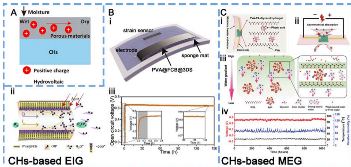
Fig. 13. CHs-based hydrovoltaics (evaporation-induced generators, EIGs; moisture-induced generators, MEGs). (A) The working mechanism of CHs-based EIGs. (B) i) Schematic diagram, ii) working principle, and electrical output iii) of a superabsorbent hydrogels-based EIG. Reproduced from ref. [342] with permission from Elsevier, copyright 2020. (C) i) Structure of a CH-MEG device with asymmetric-moisture penetration layers. ii) Schematic diagram of the asymmetric moisture stimulus-induced potential in the MEG. iii) The proposed mechanism of moisture-induced ionic diffusion process. iv) The continuous voltage output of an MEG device under open ambient environment. Reproduced from ref. [347] with permission from Wiley-VCH, copyright 2022.
