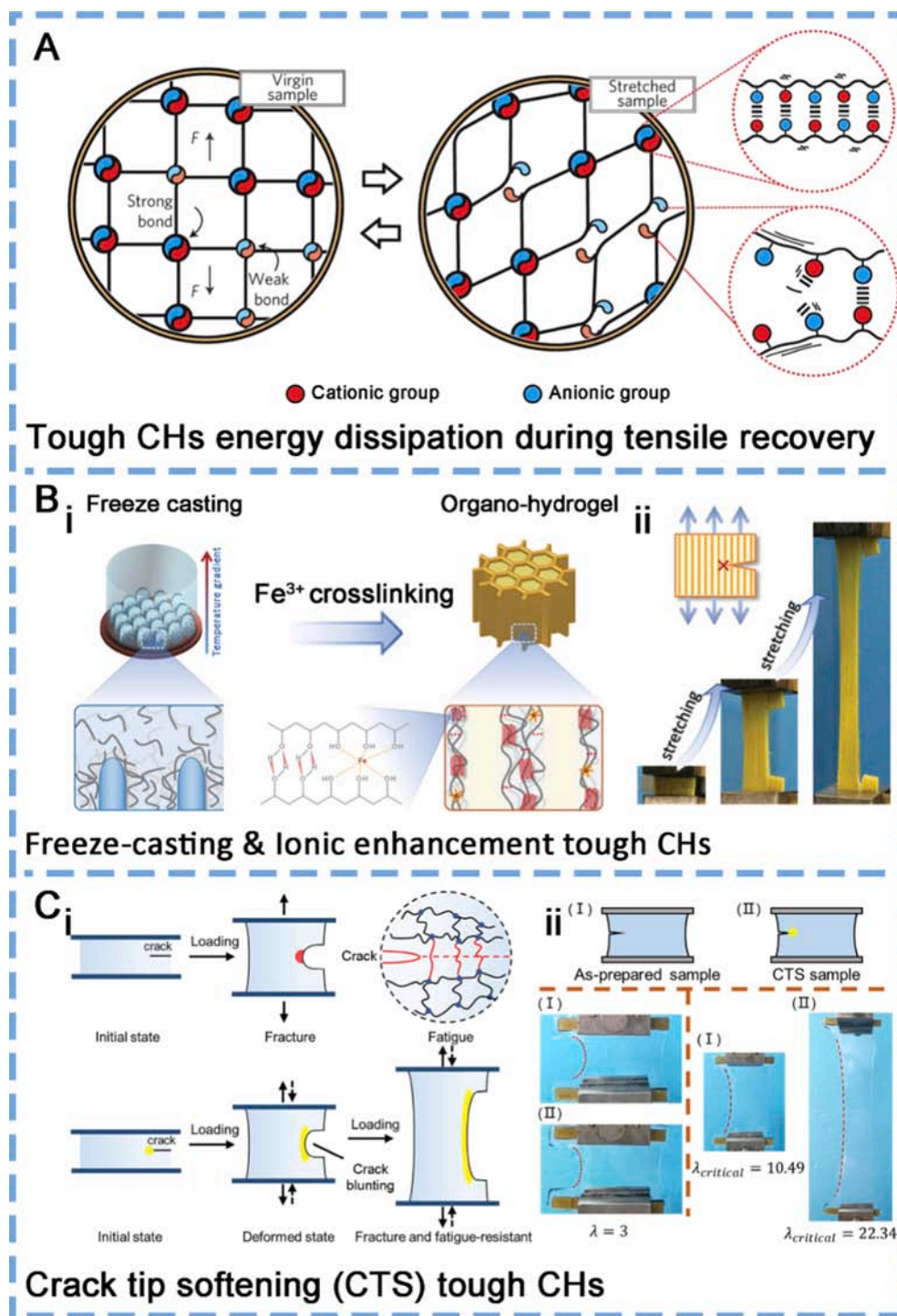
Fig. 8. Toughness and state-of-the-art methods to composite tough CHs. (A) Illustration of polymer networks with different strength. Reproduced from ref. [221] with permission from Springer Nature Limited, copyright 2013. (B) i) Schematic diagrams of freeze-casting assisted solution substitution strategy of the PVA organoCH. ii) Images of a sample being stretched. Reproduced from ref. [226] with permission from Wiley-VCH, copyright 2022. (C) i) Schematic illustration of crack tip softening makes the hydrogel crack blunt and resists the crack propagation under both monotonic load and cyclic load. ii) Images of crack blunting in the as-prepared and CTS hydrogel samples. Reproduced from ref. [230] with permission from Proceedings of the National Academy of Sciences, copyright 2023.
