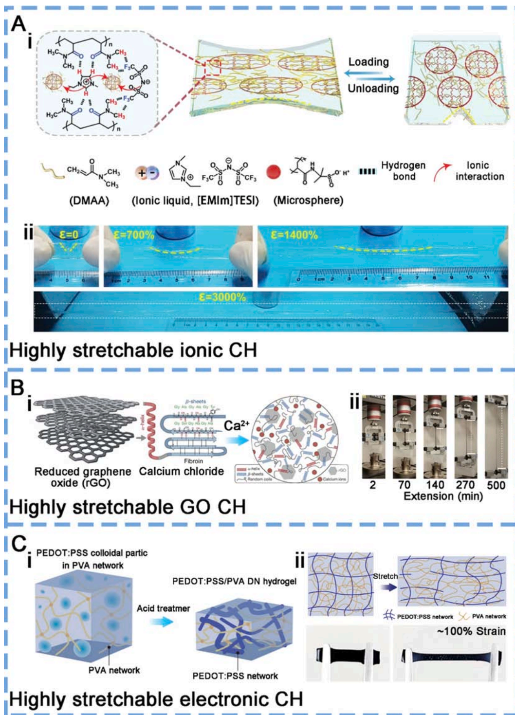
Fig. 5. Representative methods to improve stretchability. (A) Stretchable ionic CHs. i) Schematic illustration of ionogels. iii) Images of the stretch process from 0 to 3000%. Reproduced from ref. [166] with permission from Wiley-VCH, copyright 2022. (B) Highly stretchable GO CHs. i) The components used for preparation of these CHs. ii) Photographic images showing tensile stretching of CHs with an Instron mechanical tester. Reproduced from ref. [15] with permission from Wiley-VCH, copyright 2022. (C) Stretchable electronic CHs. i) Schematic illustration of the fabrication and structural change of PEDOT:PSS and PVA acid treatment process. ii) Schematic illustration of the deformation mechanism of the PEDOT:PSS/PVA DN hydrogel and images of DN hydrogel under stretching. Reproduced from ref. [169] with permission from Wiley-VCH, copyright 2022.
