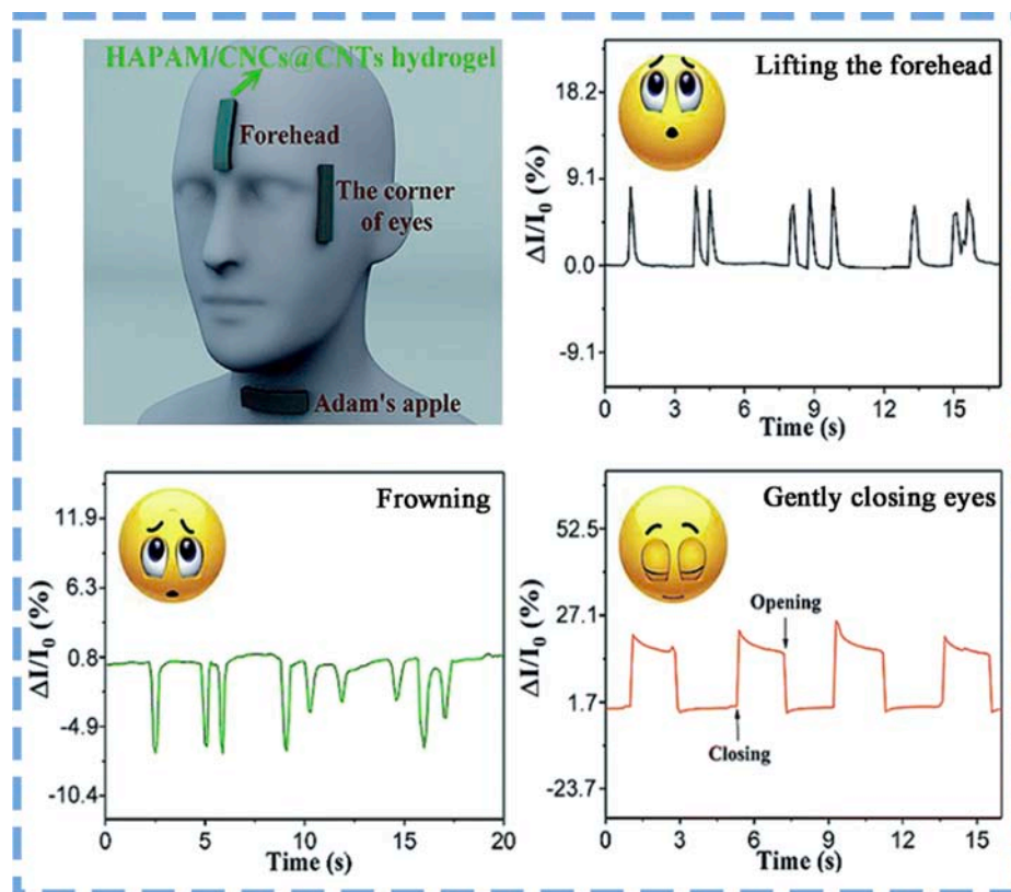
Fig. 16. CHs-based highly sensitive strain sensor attached to the forehead, the corner of the eye to detect facial expressions and corresponding current responses. Reproduced and reprinted with permission. Reproduced from ref. [395] with permission from The Royal Society of Chemistry, copyright 2019.
