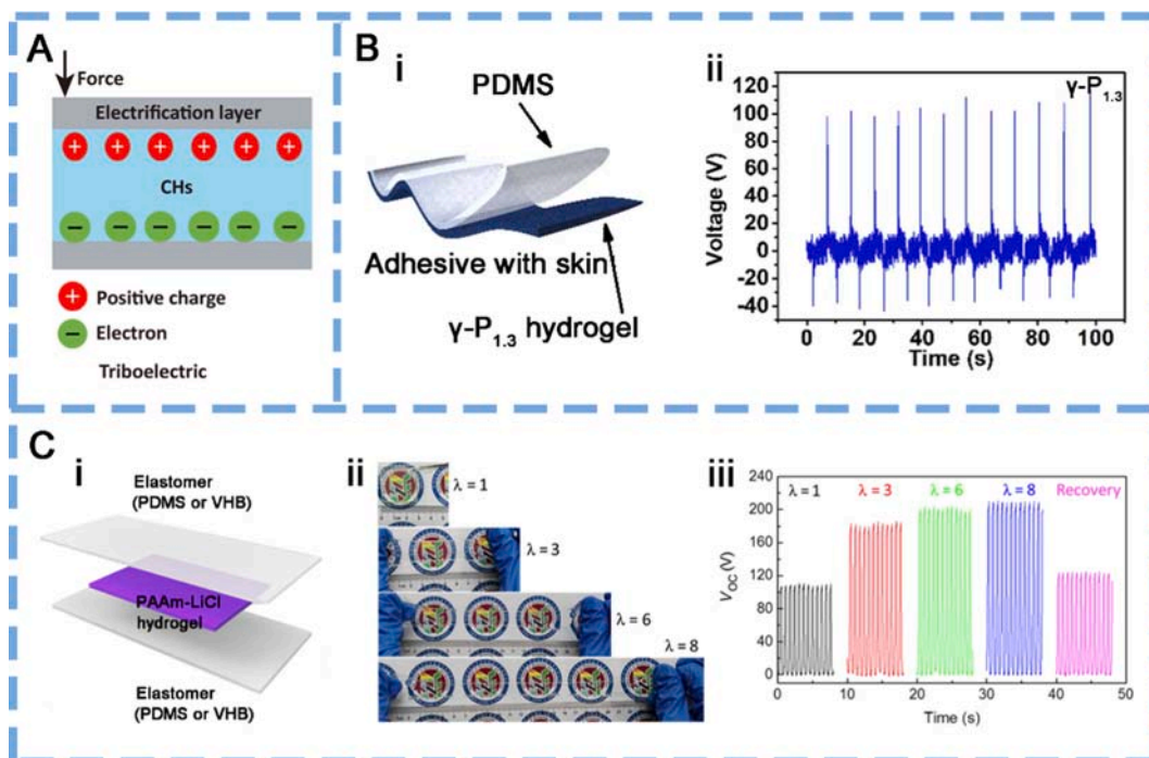
Fig. 11. CHs-based TENGs. (A) Working mechanism. (B) i) Schematic diagram of the architecture for TENG. ii) Output voltage of TENG. \gamma -polyglutamic acid/1.3 wt% PEDOT:PSS ( \gamma -P 1.3 ). Reproduced from ref. [67] with permission from Elsevier, copyright 2022. (C) i) Structure of CHs-based single-electrode TENG for bioenergy harvesting. ii) Images of the TENG at different stretched states and iii) its corresponding output. Reproduced from ref. [301] with permission from American Association for the Advancement of Science, copyright 2017.
